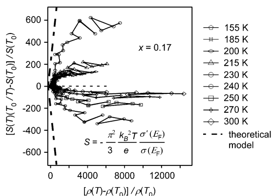
Figure 4. Correlation between thermoelectric power S(T) and resistivity \rho(T) . Relative changes of \Delta S/S_0 versus \Delta\rho/\rho_0 in the natural sample with x=0.17 at various temperatures ( T_0=155, 185, 200, 215, 230, 240, 250, 270 , and 300 K). The experimental data substantially deviate from the linear relationship predicted by Mott's formula, which is indicated by the dotted line.
